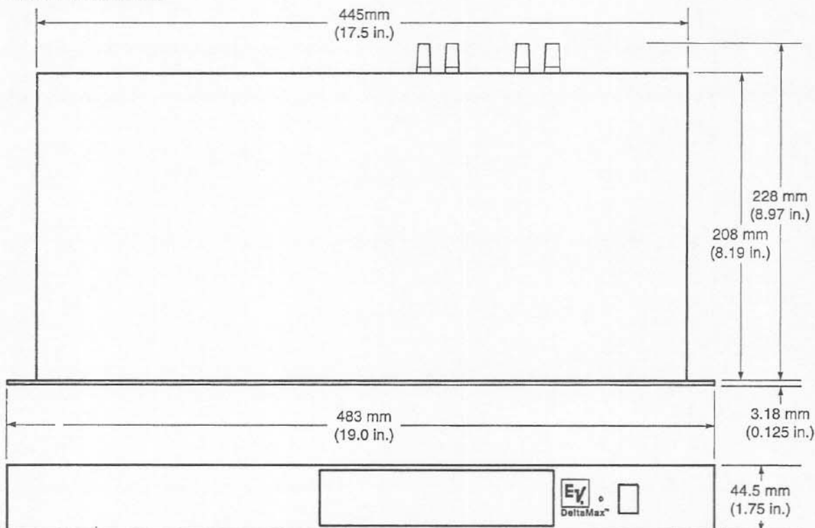
FIGURE 3 — DMC-2181S Dimensions
